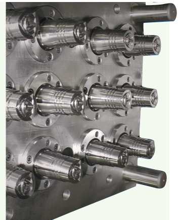
Mold-Rite retired its 20-year-old tools and built new ones with dovetail collapsible cores after finding that the cost was justified through overall savings.
